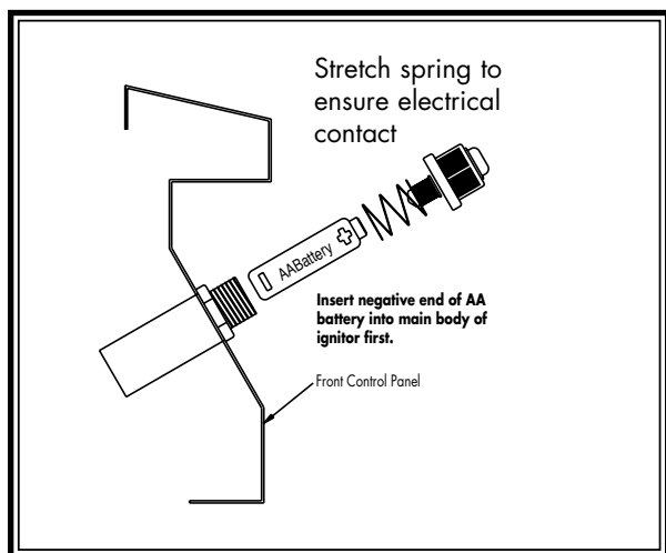
Figure 1 Igniter Battery Installation Instructions:
